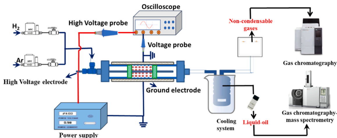
Fig. 1. Schematic diagram for plasma-catalytic upcycling of polyethylene waste reaction.
