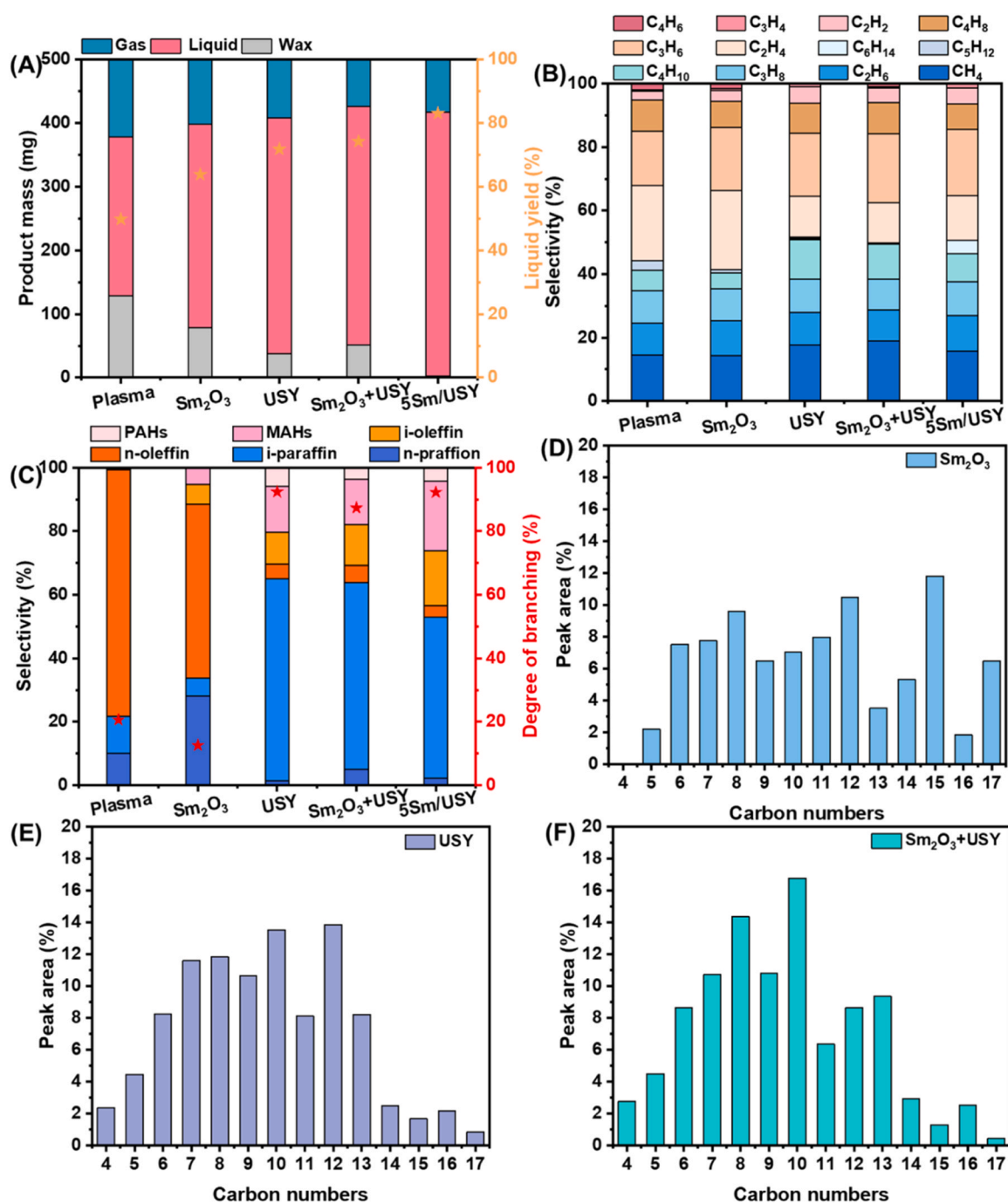
Fig. 6. Plasma-catalytic performance of \text{Sm}_2\text{O}_3 , USY, \text{Sm}_2\text{O}_3 +USY and 5Sm/USY catalysts: (A) product mass, (B) the selectivity of different components in gaseous product, (C) the selectivity of different components in liquid product and (D-F) carbon number distribution in liquid product. (Reaction conditions: 0.5 g LDPE, 0.2 g catalyst, input power of ca. 56 W, 30 mL/min, \text{H}_2 :Ar=3:7, 1 h, without external heating, ambient pressure.).
