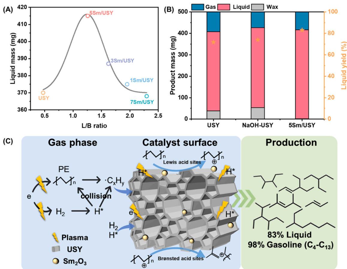
Fig. 7. (A) Liquid mass over L/B ratio of xSm/USY catalysts and (B) Product mass of plasma-catalytic performance over USY, NaOH-USY and 5Sm/USY catalysts. (Reaction conditions: 0.5 g plastics, 0.2 g catalyst, input power of ca. 56 W, 30 mL/min, \text{H}_2 :Ar=3:7, 1 h.) (C) A possible mechanism of plasma-catalytic LDPE upcycling over the 5Sm/USY catalyst without external heating.
