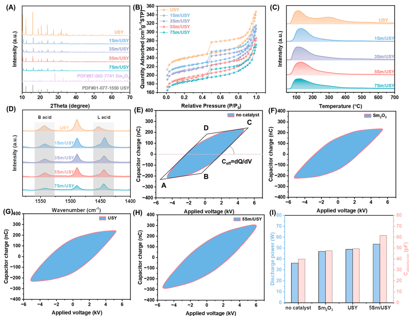
Fig. 2. (A) XRD patterns, (B) N_2 adsorption-desorption isotherms, (C) NH_3 -TPD profiles and (D) Py-IR spectra measured at 150 °C of Sm/USY catalysts with different Sm loadings. Q-U Lissajous figures of (E) no catalyst, (F) Sm_2O_3 catalyst, (G) USY catalyst and (H) 5Sm/USY catalyst in plasma-catalytic reaction. (I) Discharge power and effective capacitance of no catalyst, Sm_2O_3 catalyst, USY catalyst and 5Sm/USY catalyst in plasma-catalytic reaction. (Reaction conditions: 0.5 g LDPE, 0.2 g catalyst, input power of ca. 56 W, 30 mL/min, H_2 : Ar=3:7, 1 h, without external heating, ambient pressure.).
