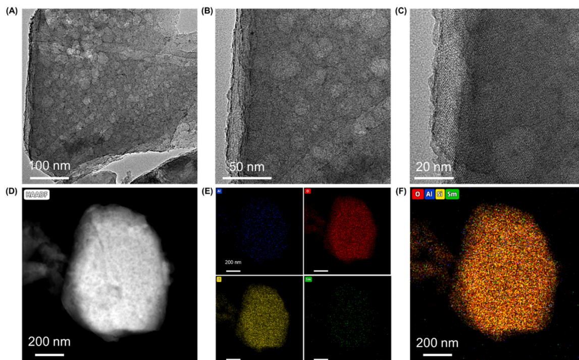
Fig. 3. (A-C) TEM images and (D-F) the corresponding mapping of 5Sm/USY catalysts.
