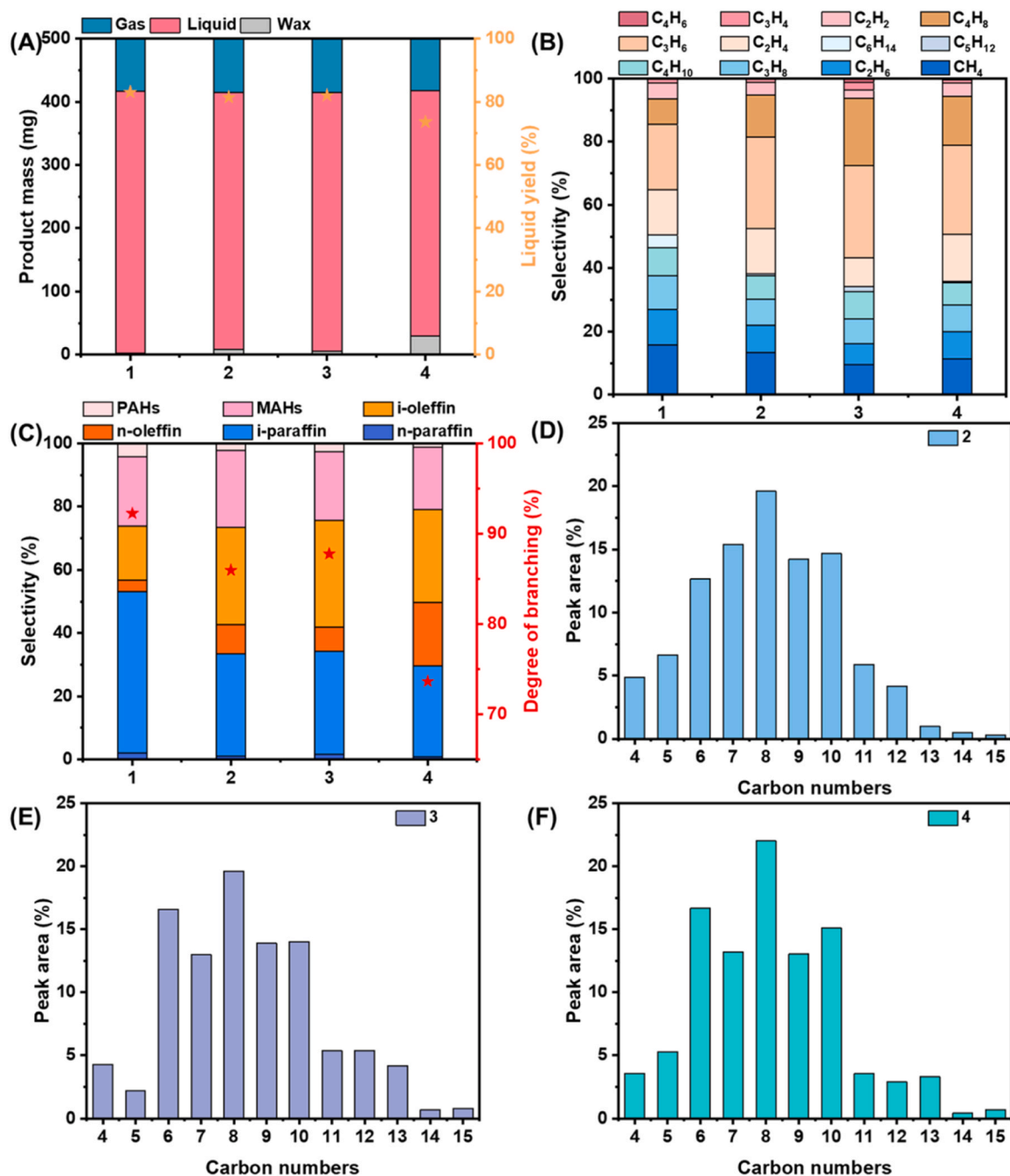
Fig. 8. Plasma-catalytic performance of successive cycles over 5Sm/USY catalyst: (A) product mass, (B) the selectivity of different components in gaseous product, (C) the selectivity of different components in liquid product and (D-F) carbon number distribution in liquid product. (Reaction conditions: 0.5 g plastics, 0.2 g catalyst, input power of ca. 56 W, 30 mL/min, H_2:Ar=3:7 , 1 h, without external heating, ambient pressure.).
