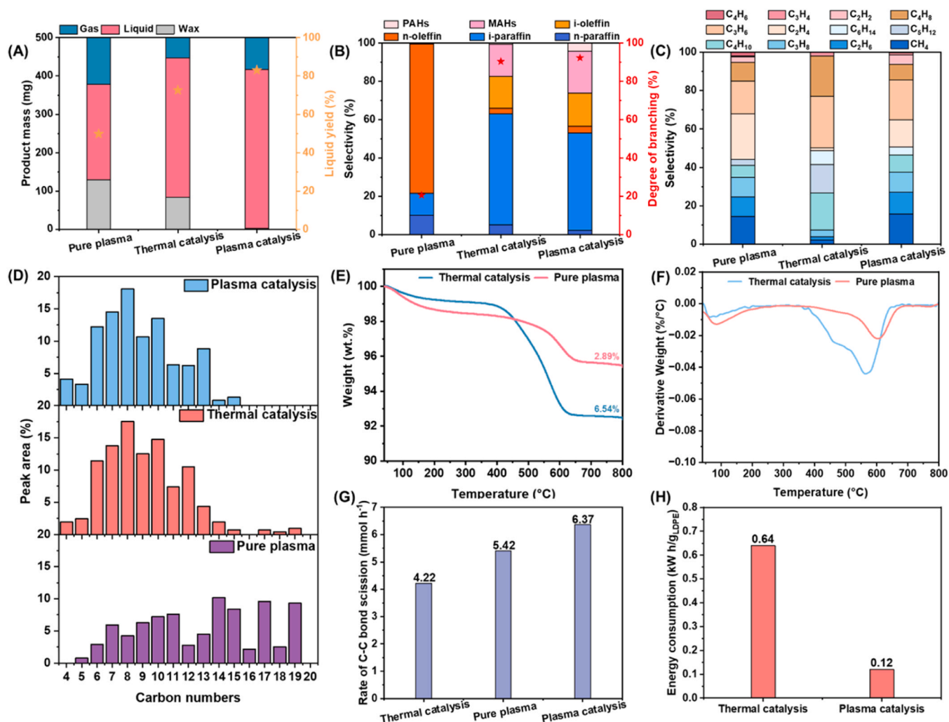
Fig. 5. Pure plasma performance, thermal catalysis and plasma catalysis performance over 5Sm/USY catalyst: (A) product weight, (B) the selectivity of different components in liquid product, (C) the selectivity of different components in gaseous product, (D) carbon number distribution in liquid product. (E) TG and (F) DTG curves of spent 5Sm/USY catalysts, (G) rate of C-C bond scission of plasma, thermal catalysis and plasma catalysis and (H) electricity consumption of thermal catalysis and plasma catalysis over 5Sm/USY catalyst. (Reaction conditions of plasma: 0.5 g LDPE, 0.2 g catalyst or not, input power of ca. 56 W, 30 mL/min, H 2 : Ar=3:7, 1 h, without external heating, ambient pressure. Reaction conditions of pyrolysis: 0.5 g LDPE, 0.2 g catalyst, 30 mL/min, 550°C, 1 h.).
