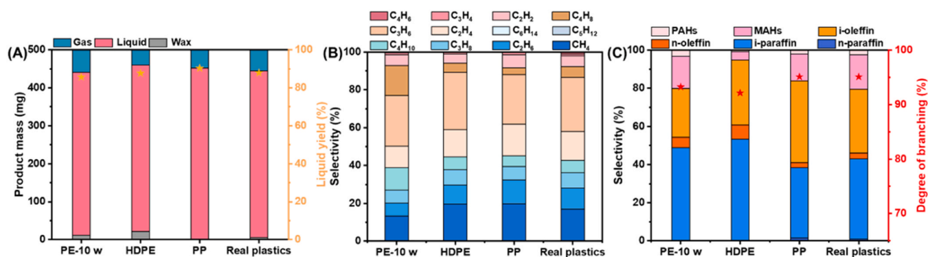
Fig. 9. Plasma-catalytic performance of different plastics over 5Sm/USY catalyst: (A) product mass, (B) the selectivity of different components in gaseous product, (C) the selectivity of different components in liquid product. (Reaction conditions: 0.5 g plastics, 0.2 g catalyst, input power of ca. 56 W, 30 mL/min, H 2 :Ar=3:7, 1 h, without external heating, ambient pressure.).
