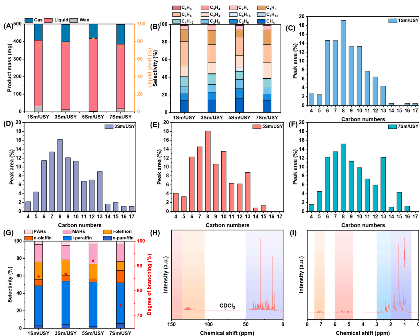
Fig. 4. Plasma-catalytic performance of Sm/USY catalysts with different Sm loadings: (A) product mass, (B) the selectivity of different components in gaseous product, (C-F) carbon number distribution in liquid product, (G) the selectivity of different components in liquid product. (H) ^{13}\text{C} NMR and (I) ^1\text{H} NMR spectra of liquid products over 5Sm/USY catalyst for plasma-catalytic LDPE hydrogenolysis. (Reaction conditions: 0.5 g LDPE, 0.2 g catalyst, input power of ca. 56 W, 30 mL/min, \text{H}_2 :Ar=3:7, 1 h, without external heating, ambient pressure.).
